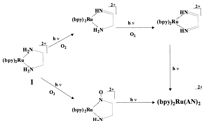
Scheme 1. Photoreaction pathway of [\text{Ru}(\text{bpy})_2(\text{en})](\text{PF}_6)_2 in acetonitrile.
